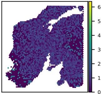
SNU24A FBXO42 expression Moran's I = 0.05
