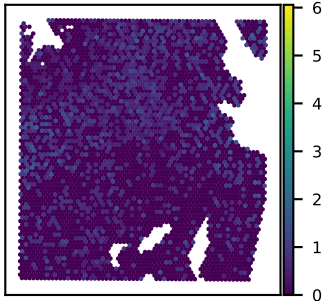
SNU51A PTPRB expression Moran's I = 0.07
