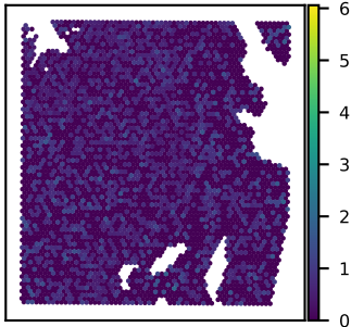
SNU51A CLEC16A expression Moran's I = 0.01
