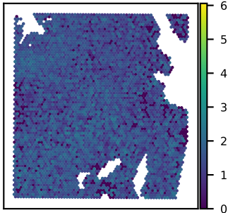
SNU51A GANAB expression Moran's I = 0.10
