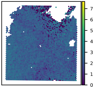
SNU21B YWHAQ expression Moran's I = 0.17
