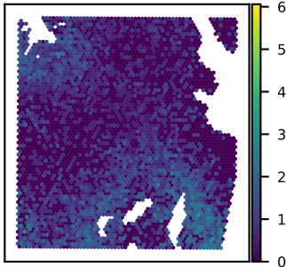
SNU51A FCGBP expression Moran's I = 0.40
