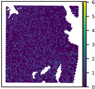
SNU51A C17orf58 expression Moran's I = 0.03
