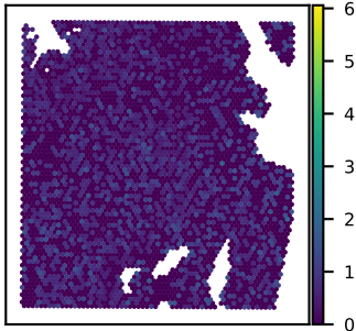
SNU51A C12orf45 expression Moran's I = -0.00
