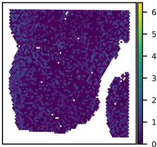
SNU25B CREB3L2 expression Moran's I = 0.06
