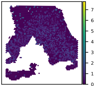
SNU18A TNFSF14 expression Moran's I = 0.13
