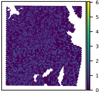
SNU51A CEP57L1 expression Moran's I = 0.02
