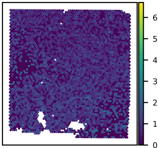
SNU43A HRAS expression Moran's I = 0.05
