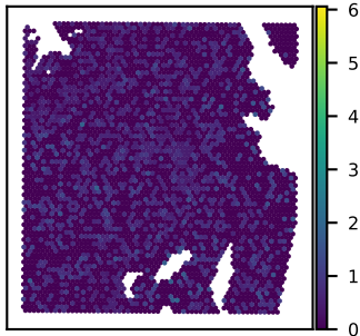
SNU51A PUS7L expression Moran's I = 0.01
