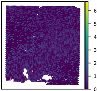
SNU43A SMARCD1 expression Moran's I = 0.02
