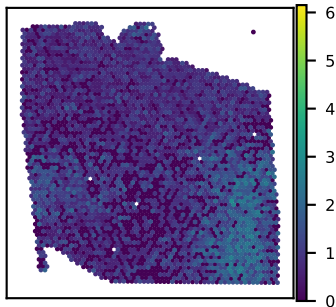
SNU27A EFHD2 expression Moran's I = 0.28
