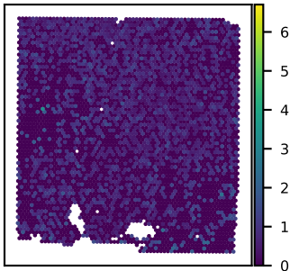
SNU43A SLCO3A1 expression Moran's I = 0.04
