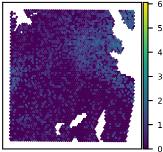
SNU51A C1orf115 expression Moran's I = 0.35
