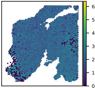
SNU24A HNRNPH1 expression Moran's I = 0.09
