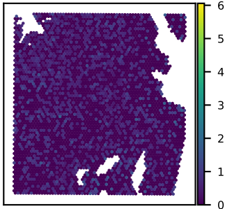
SNU51A ZNF397 expression Moran's I = 0.02
