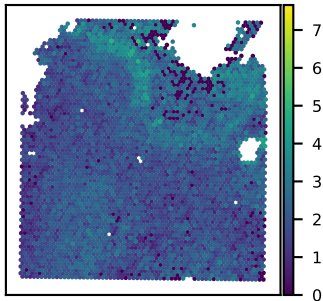
SNU21B SERPINE1 expression Moran's I = 0.36
