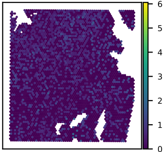
SNU51A CPQ expression Moran's I = 0.02
