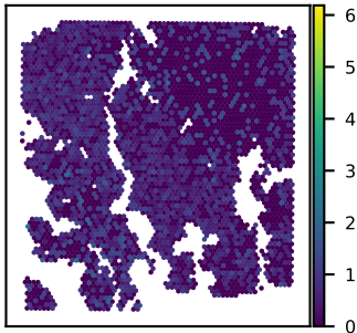
SNU16B LCORL expression Moran's I = 0.05
