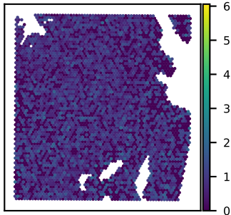
SNU51A GPBP1L1 expression Moran's I = 0.02
