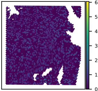
SNU51A CISD2 expression Moran's I = 0.02
