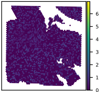
SNU24B WDR35 expression Moran's I = 0.01
