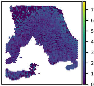
SNU18A TMEM132A expression Moran's I = 0.18
