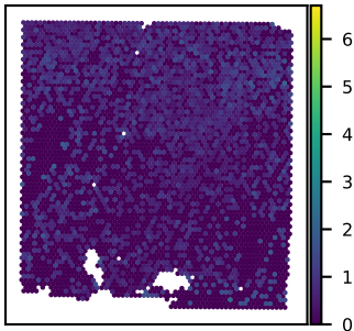
SNU43A CHST15 expression Moran's I = 0.10
