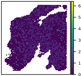
SNU24A RADX expression Moran's I = 0.03
