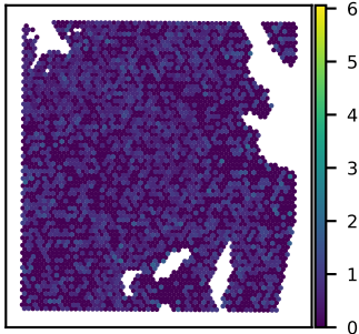
SNU51A INPPL1 expression Moran's I = 0.02
