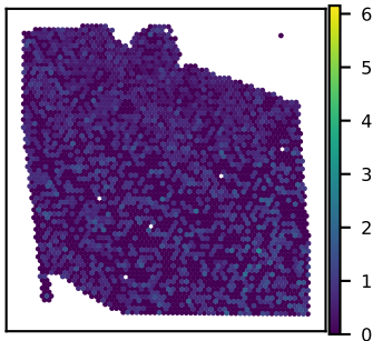
SNU27A BRI3BP expression Moran's I = 0.01
