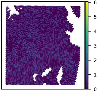
SNU51A PPP4R1 expression Moran's I = 0.03
