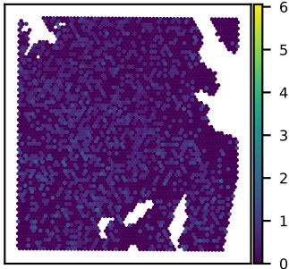
SNU51A TSPAN11 expression Moran's I = 0.03
