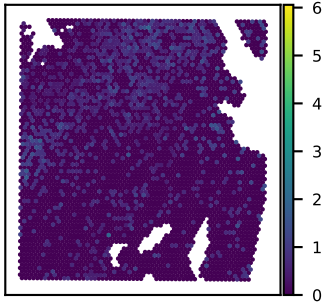
SNU51A CIITA expression Moran's I = 0.15
