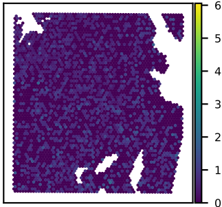
SNU51A ZBTB45 expression Moran's I = 0.01
