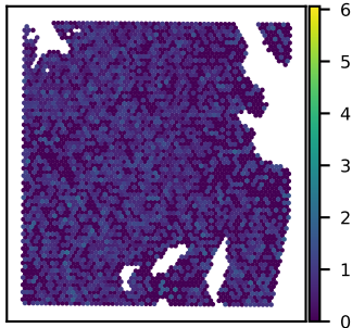
SNU51A UGGT1 expression Moran's I = 0.04
