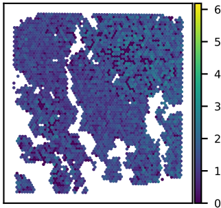
SNU16B GABARAPL2 expression Moran's I = 0.08
