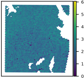
SNU51A PPP2CB expression Moran's I = 0.12
