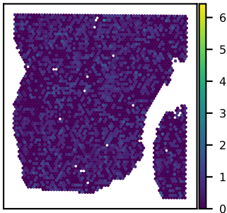
SNU25B C6orf136 expression Moran's I = 0.01
