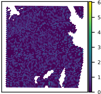
SNU51A SMARCD2 expression Moran's I = 0.01
