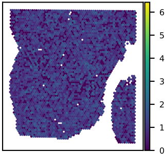
SNU25B CKAP5 expression Moran's I = 0.03
