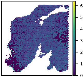
SNU24A PGRMC1 expression Moran's I = 0.15
