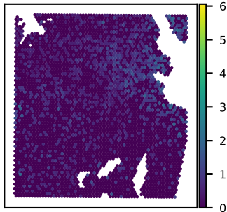
SNU51A STXBP6 expression Moran's I = 0.15
