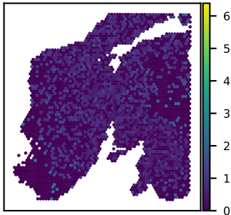
SNU24A SLC36A1 expression Moran's I = 0.03
