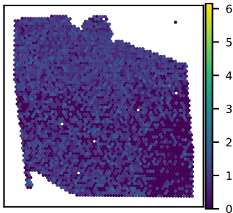
SNU27A SLC12A4 expression Moran's I = 0.14
