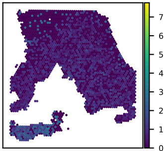
SNU18A SLC1A4 expression Moran's I = 0.18
