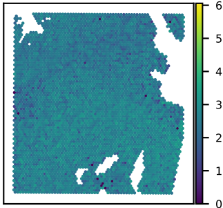
SNU51A HNRNPDL expression Moran's I = 0.18
