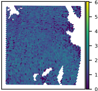
SNU51A VASH1 expression Moran's I = 0.16
