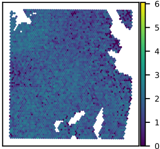
SNU51A KDEL2 expression Moran's I = 0.20
