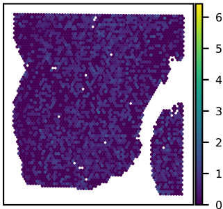
SNU25B CACNB3 expression Moran's I = 0.06
