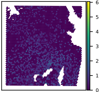
SNU51A NHLH1 expression Moran's I = 0.15
